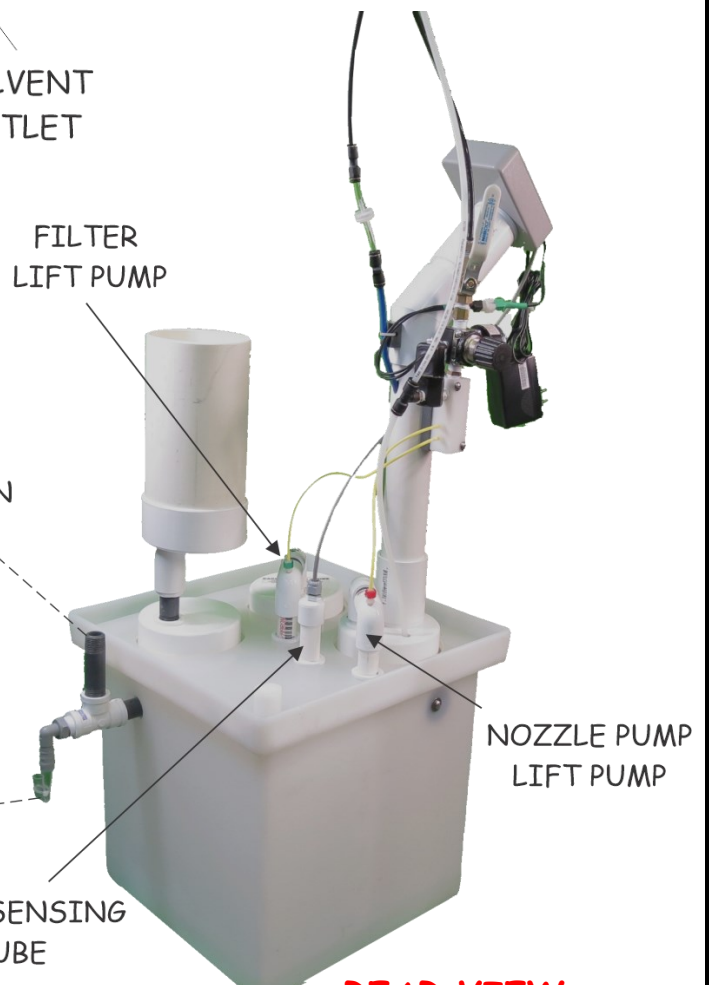
REAR VIEW
